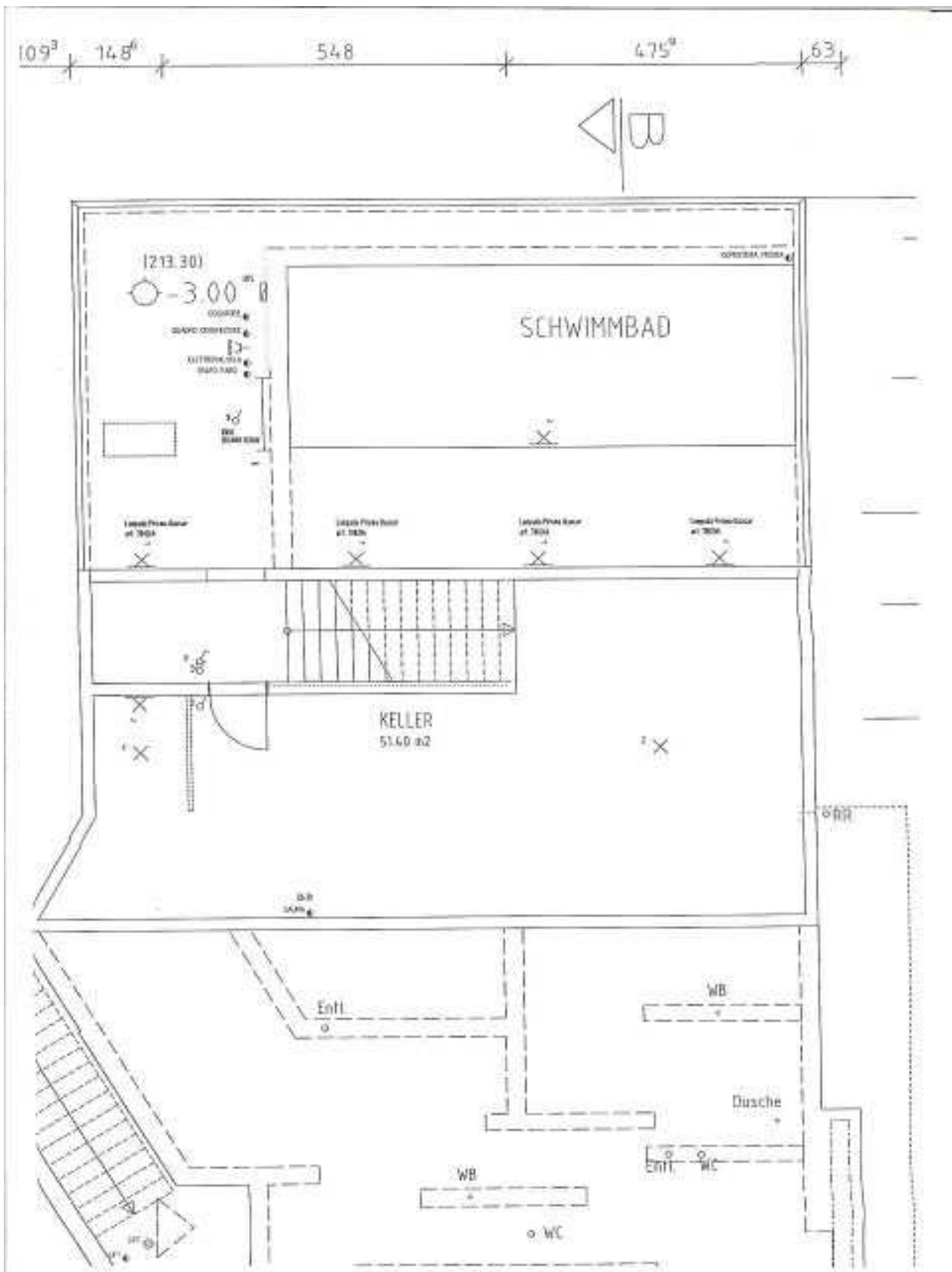
Piano PT / Grundriss Erdgeschoss
